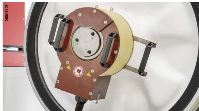
Figure 2 Rigid inductor for dismounting of wheelset bearings
