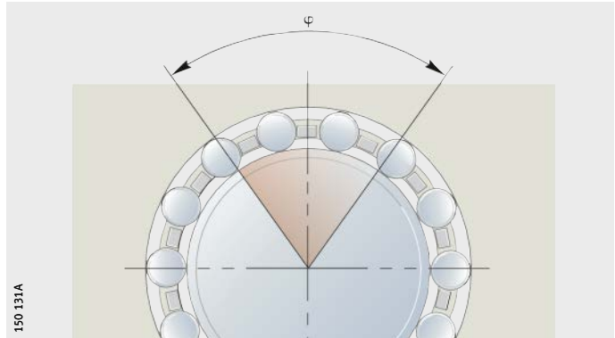
Figure 5 Swivel angle
