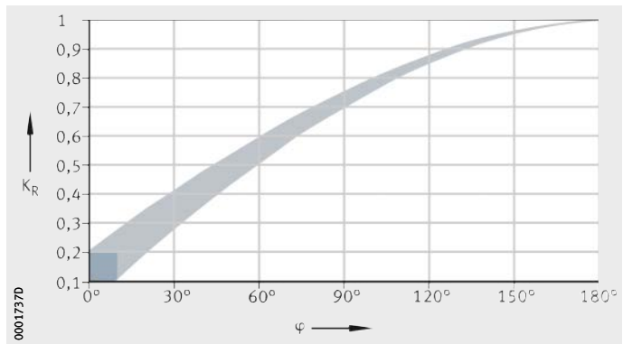
Figure 6 Oscillation factor
