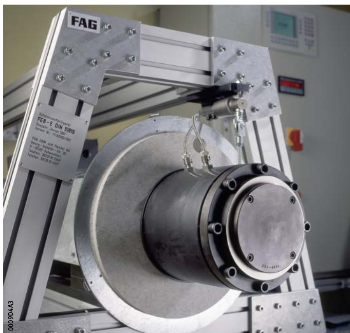
Figure 1 FE8 test rig
